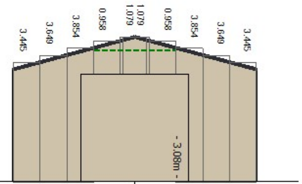
Right End
